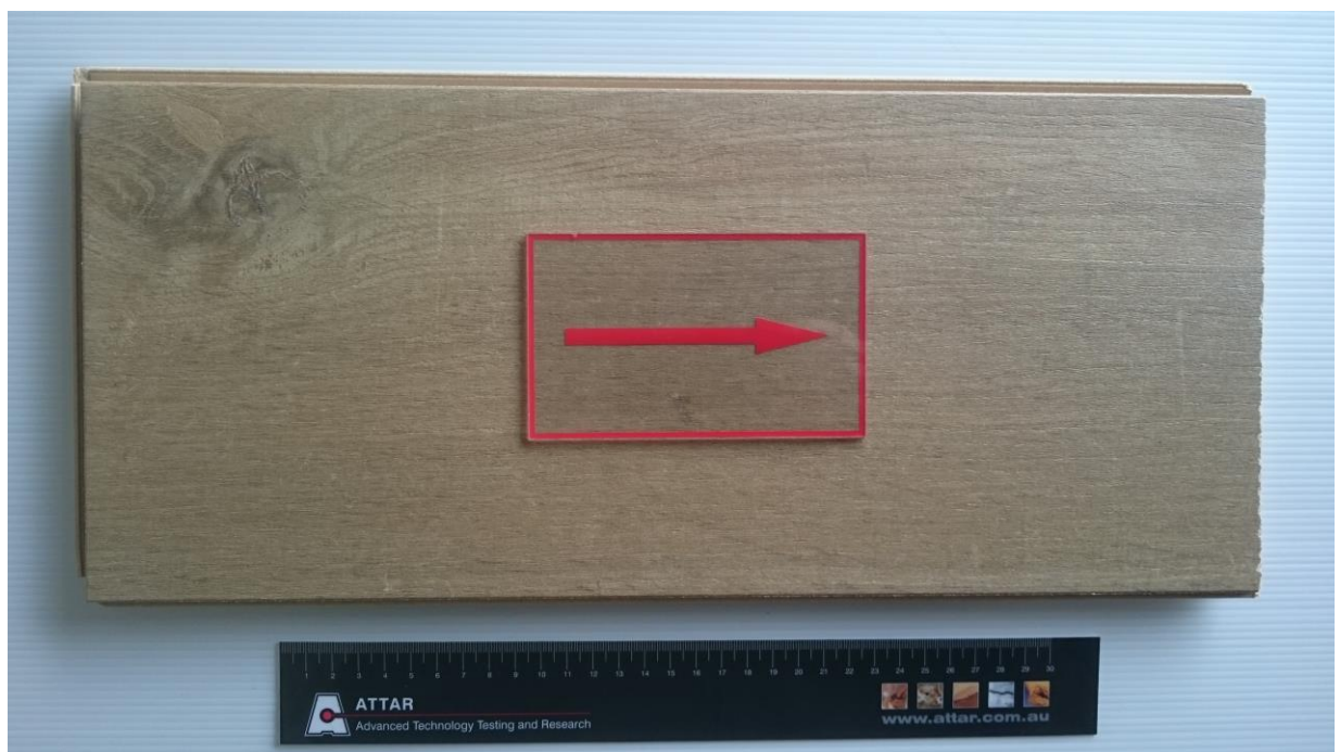
Figure 1: Quick – Step Impressive laminate flooring. Highlighted area indicates area tested and direction of test.
